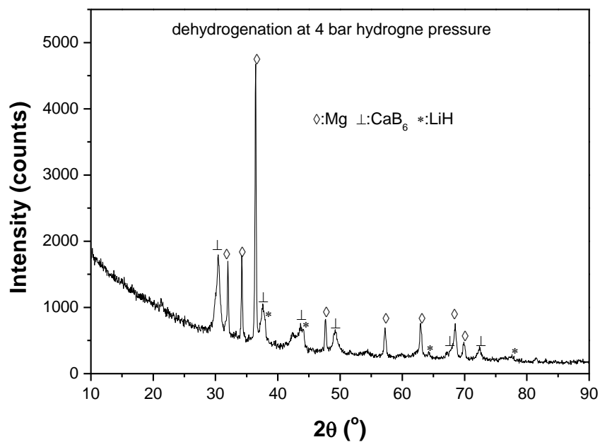
Fig. S1 XRD pattern of the dehydrogenated 6\text{LiBH}_4\text{-CaH}_2\text{-3MgH}_2 composite under 4 bar of \text{H}_2 .
