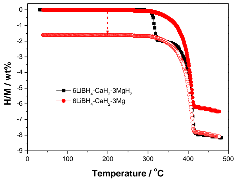
Fig. S3 Comparison on dehydrogenation behavior of the 6LiBH 4 -CaH 2 -3Mg and 6LiBH 4 -CaH 2 -3MgH 2 samples
