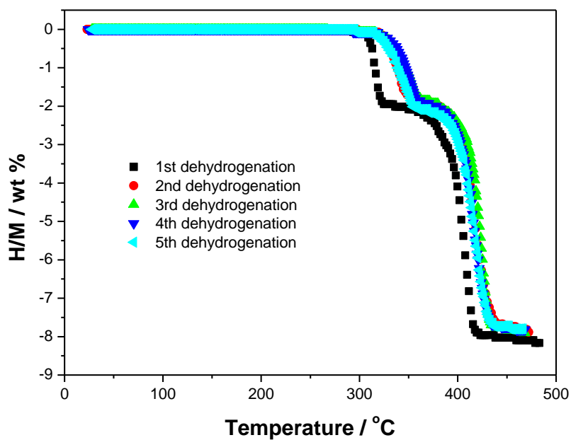
Fig. S2 Dehydrogenation curves of the 6\text{LiBH}_4\text{-CaH}_2\text{-3MgH}_2 sample in the initial five cycles
