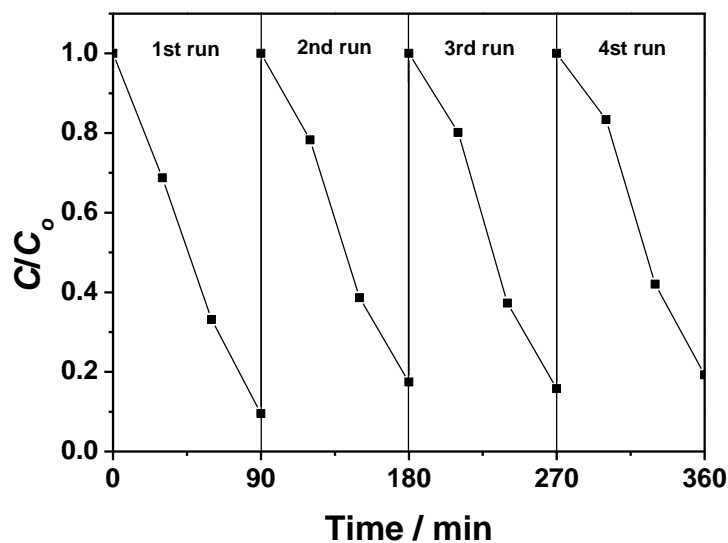
Fig. S1. Reuse activity of the sample with 1% graphene.
