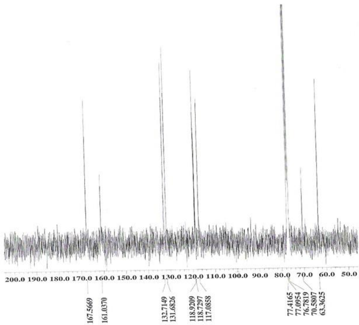
Fig 2S: ^{13}\text{C} NMR Spectrum of complex 1
