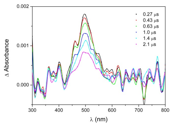
Figure S1. Triplet-singlet difference absorption spectra observed with different delays following laser excitation at 355 nm of a solution of the 1:3 Al(III)/8-HQS complex at pH 4.
