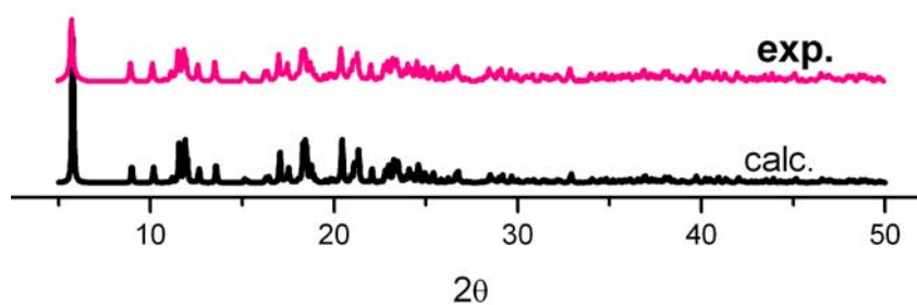
Figure S2. The experimental XRD pattern/red and the simulated XRD pattern/black from the single crystal data.
