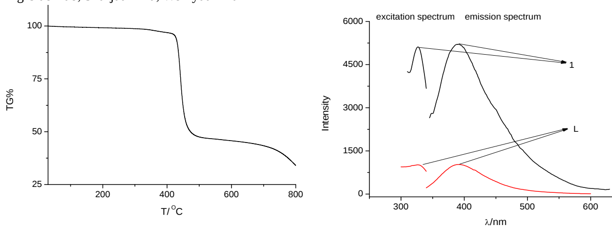
Figure S1. The TG and luminescence studies of 1 .
