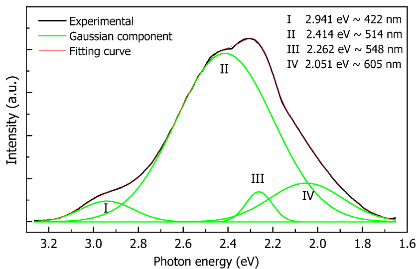
Figure S1. The emission spectrum of BLuP:0.005Eu 2+ and its Gaussian components on an energy scale.
