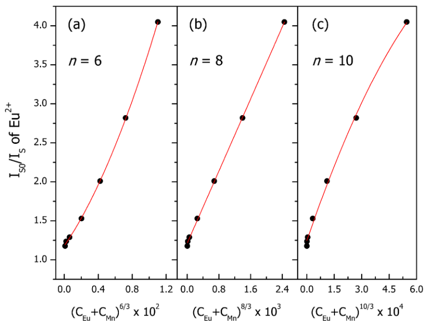
Figure S2. Dependence of I_{S0}/I_S of Eu 2+ on (a) C^{6/3} , (b) C^{8/3} , and (c) C^{10/3} .
