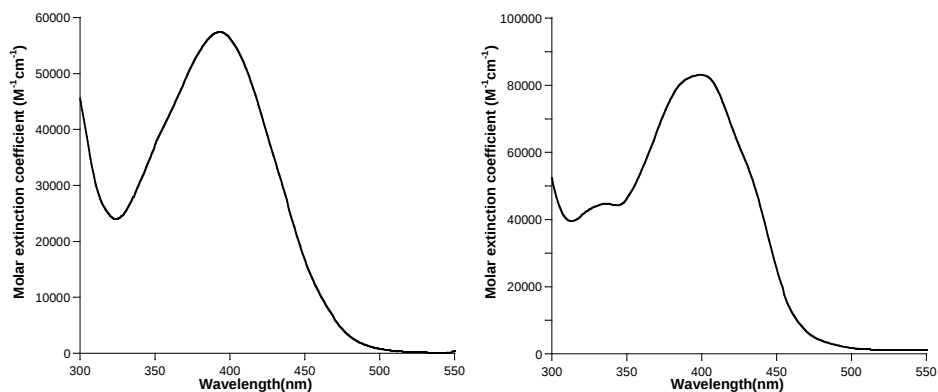
Fig. S1 Absorption spectra of complex (left) 4 and (right) 7 ( CH_2Cl_2 , 298 K).
