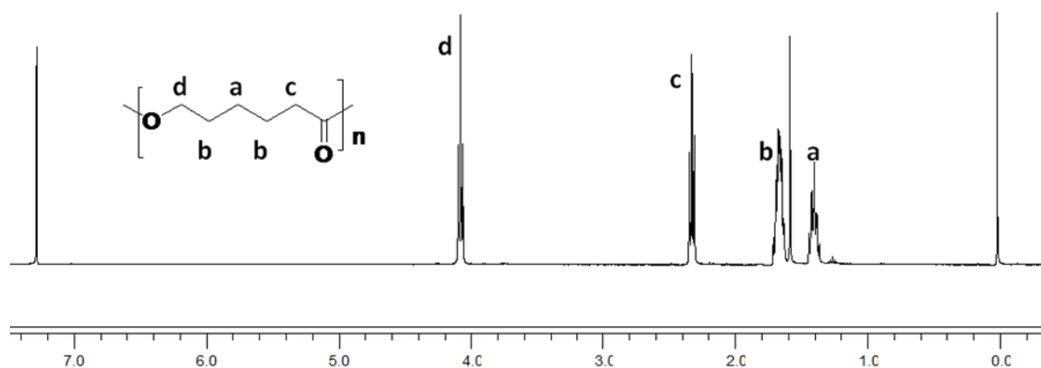
SFigure 1. ^1\text{H} NMR spectrum of PCL obtained by complex 3 (Table 3, entry 14).
