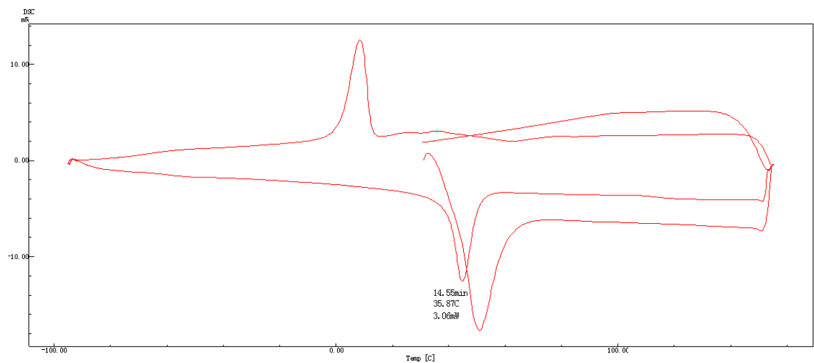
SFigure 6. DSC curve of poly(CL- co -BL) obtained by complex 3 (Table 4, entry 7).
