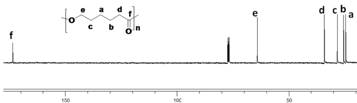
SFigure 2. ^{13}\text{C} NMR spectrum of PCL obtained by complex 3 (Table 3, entry 14).
