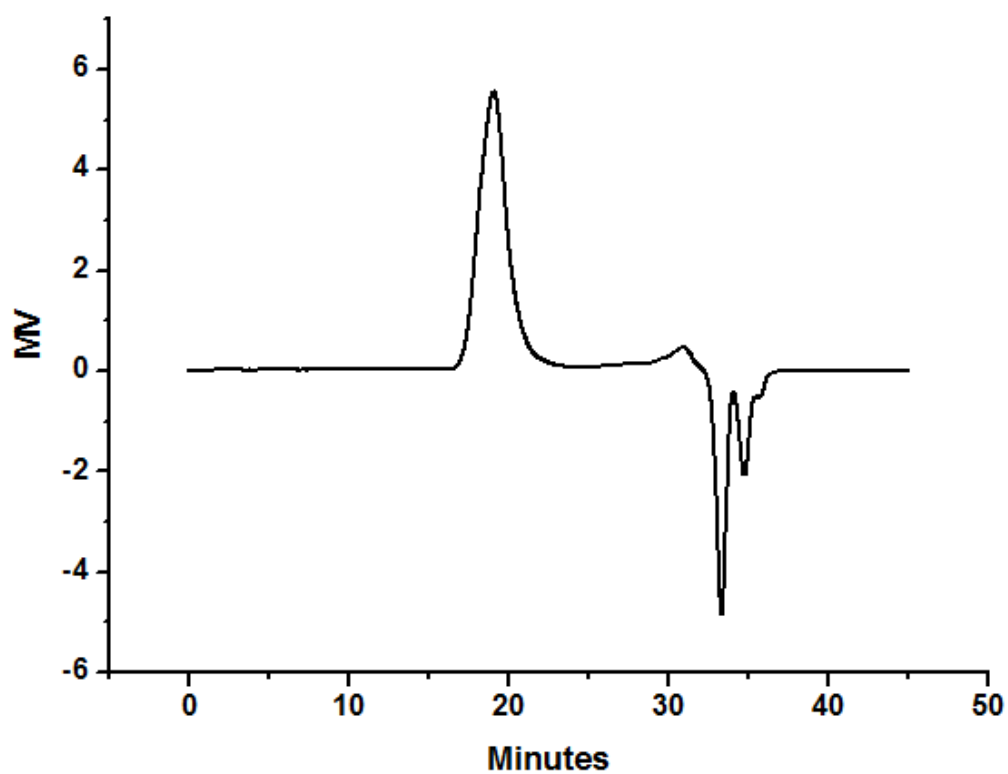
Figure 5. GPC curve of poly(CL-co-BL) obtained by complex 3 (Table 4, entry 7).
