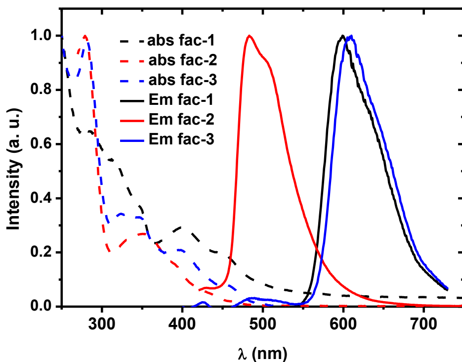
Fig. 1 Absorption (dash) and emission (solid) spectra of fac-1 (black), fac-2 (red) and fac-3 (blue) recorded in CH 2 Cl 2 at room temperature.
