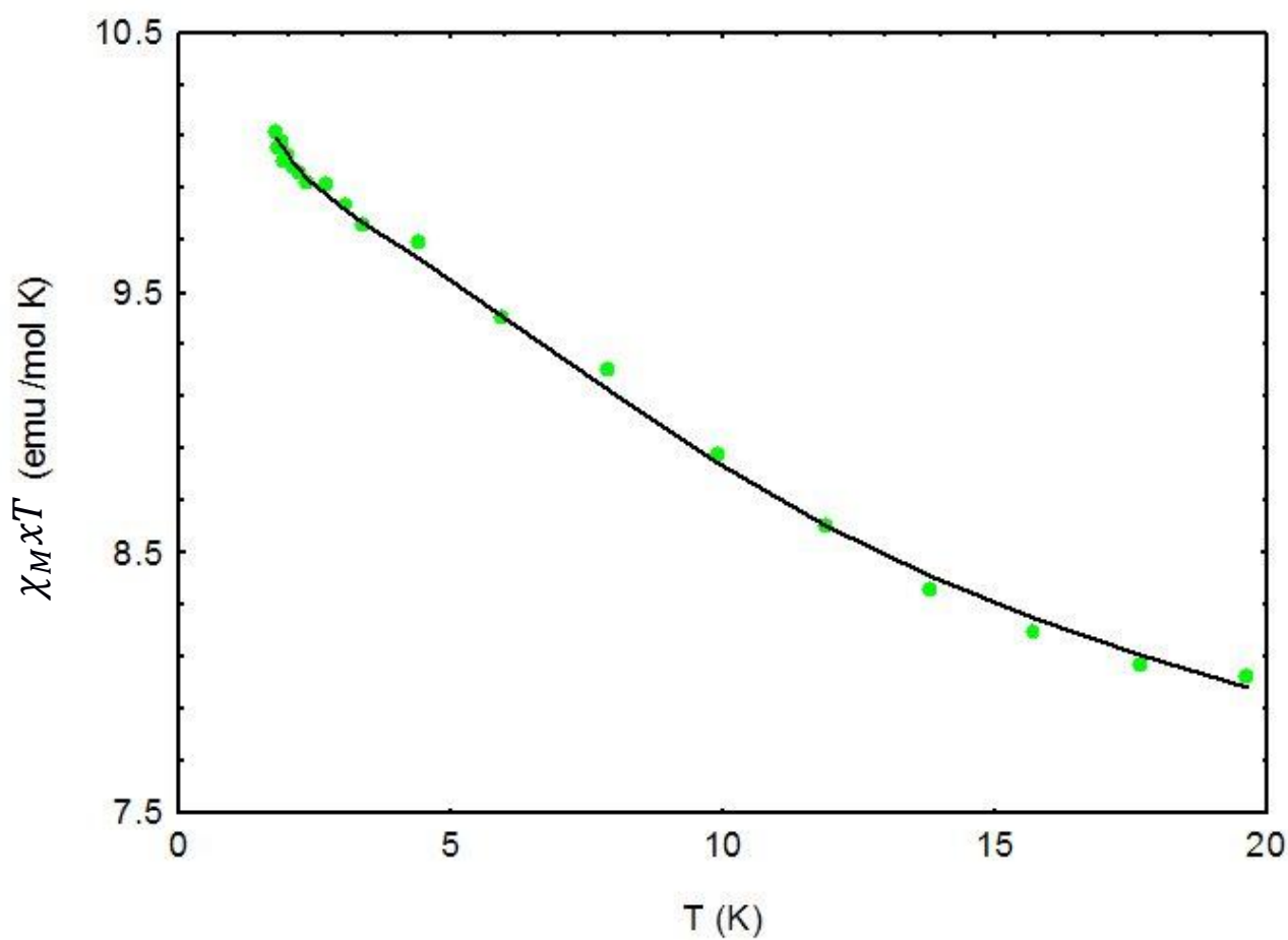
Figure S1 Thermal variation of the \chi_M x T product for \{\text{Gd}[\text{Co}(\text{H}_2\text{Maltonis})]_2\}^{3+} . The full line corresponds to the best data fit.
