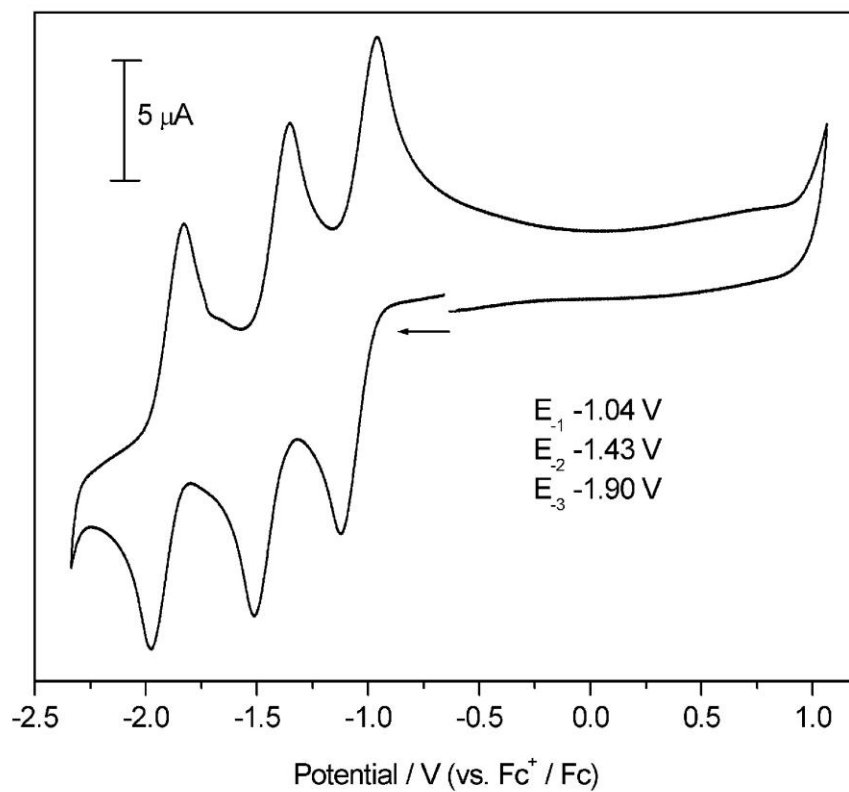
Figure S1. Cyclic voltammogram of 1.0 mM solution of \text{C}_{60} in o-DCB containing 0.2 M [\text{NnBu}_4][\text{BF}_4] at 293K
