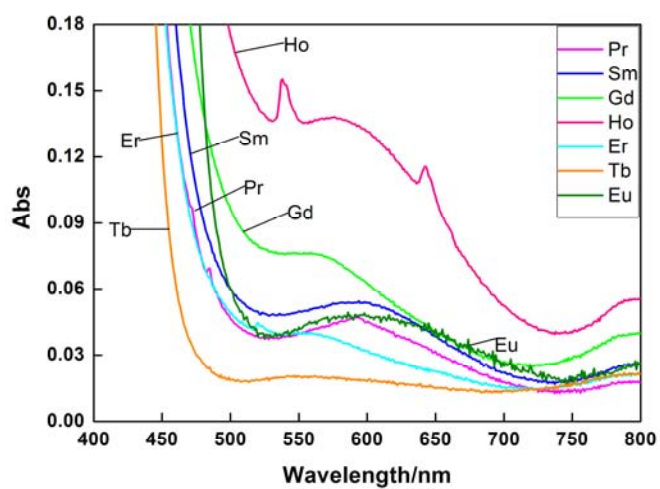
Fig. S1 UV-vis spectra of the complexes 1-7
