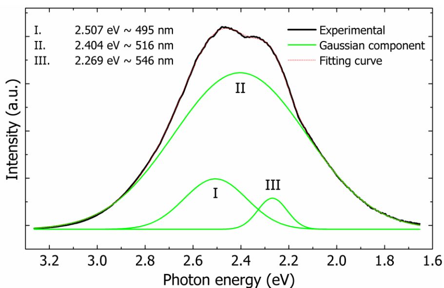
Figure S2. The emission spectrum of \text{SSP:0.005Eu}^{2+} and its Gaussian components on an energy scale. _NH
