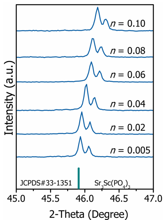
Figure S1. The details of the evolution on reflections near 2\theta = 46^\circ .
