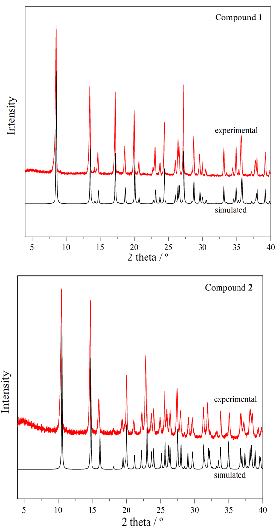
Fig. S1. Simulated (black) and experimental (red) PXRD patterns for compounds 1 (top) and 2 (bottom).
