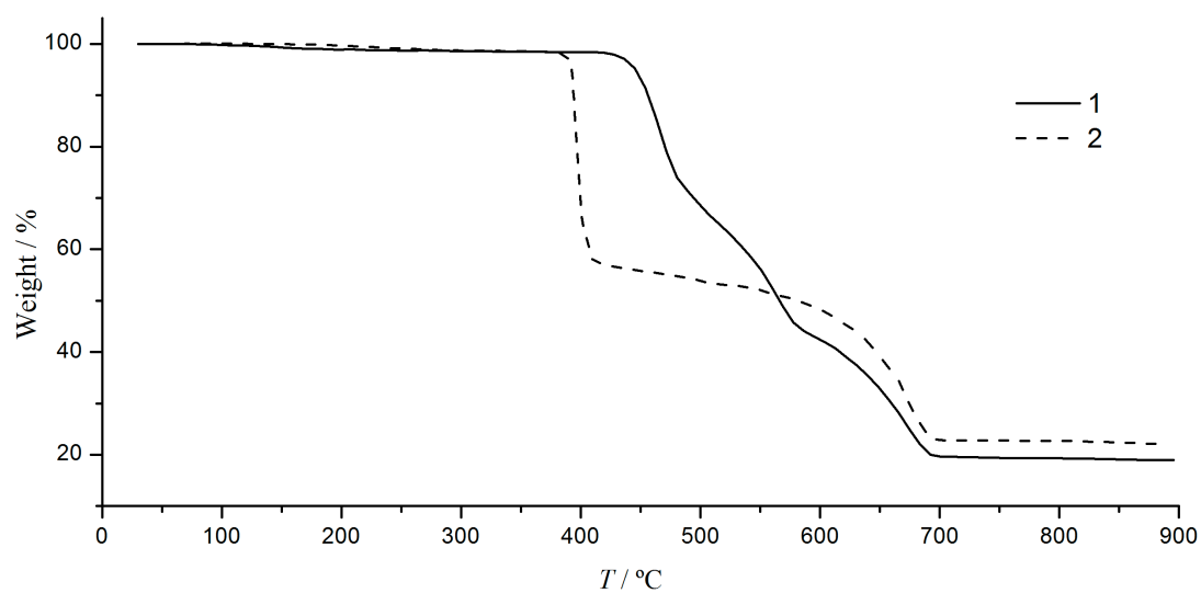
Fig. S2 TGA plots for compounds 1 (solid line) and 2 (dashed line).
