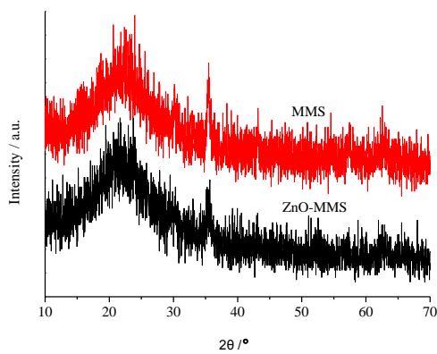
Figure S2 Wide-angle X-ray Diffraction pattern of MMS and ZnO-MMS
