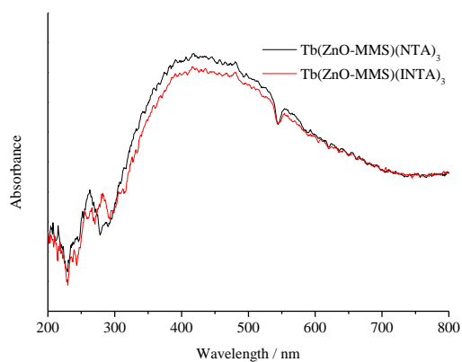
Figure S1 Ultraviolet-visible diffuse reflection absorption spectra of \text{Tb}(\text{ZnO-MMS})(\text{NTA})_3 and \text{Tb}(\text{ZnO-MMS})(\text{INTA})_3
