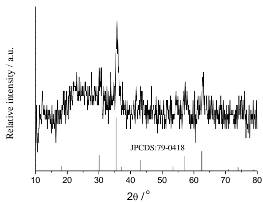
Figure S3 X-ray Diffraction pattern of \text{Fe}_3\text{O}_4 nanoparticles
