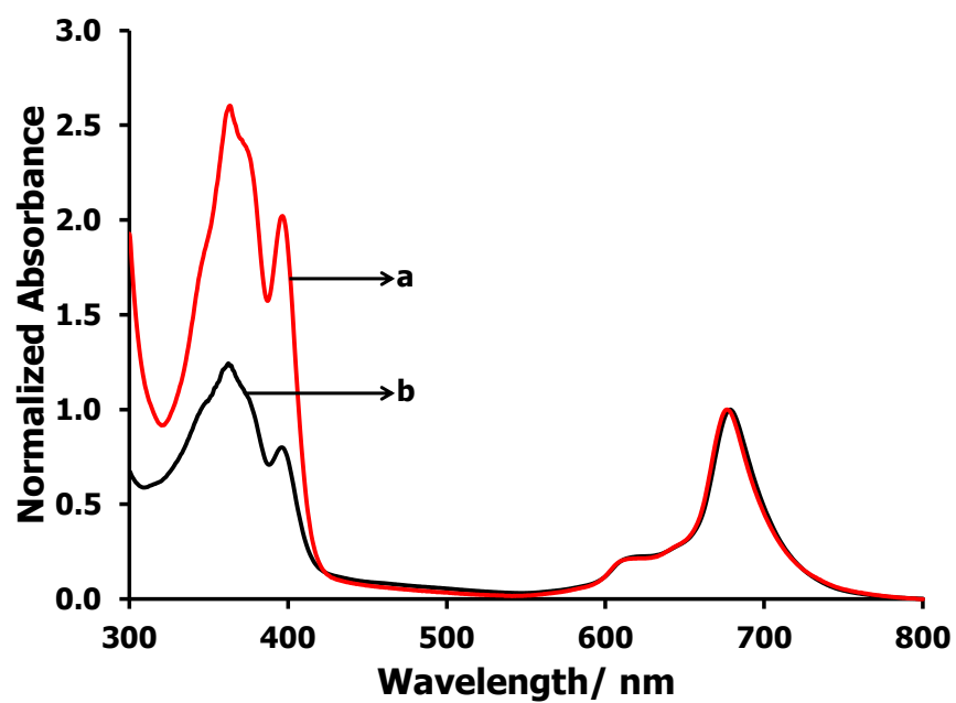
Fig. 2 UV-Vis spectra of Pc – day 1 (a) and 4 months (b) in DMSO
