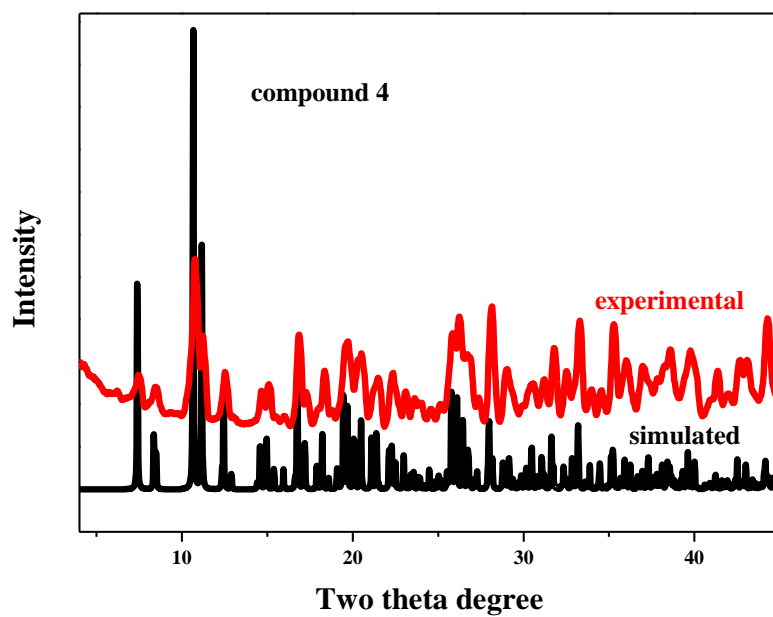
Fig. S2 The experimental (red) and simulated (black) powder XRD patterns for the title compounds.
