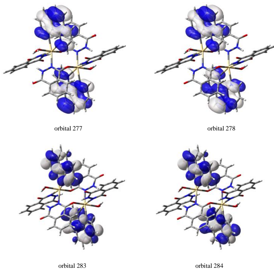
Fig. S3 The surfaces of orbitals 277, 278, 283 and 284 for compound 1.
