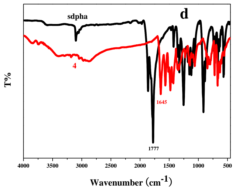
Fig. S1 The IR spectra for the title compounds and the corresponding organic acids.
