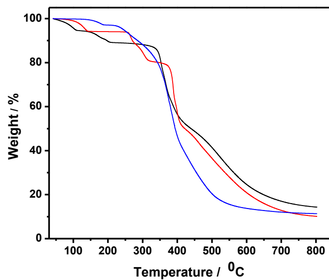
Fig. S1 TG curves of the rehydrated materials of 1 (red), 2 (blue) and 3 (black).
