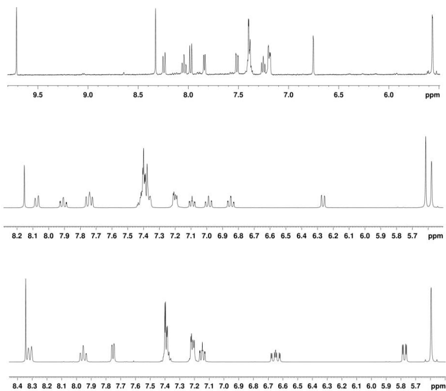
Fig S1. ^1\text{H} NMR spectra in of 1 (top), 2 (middle) and 3 (bottom) in \text{d}_3\text{-MeCN} (400 MHz, Bruker 400 AVIII spectrometer)
