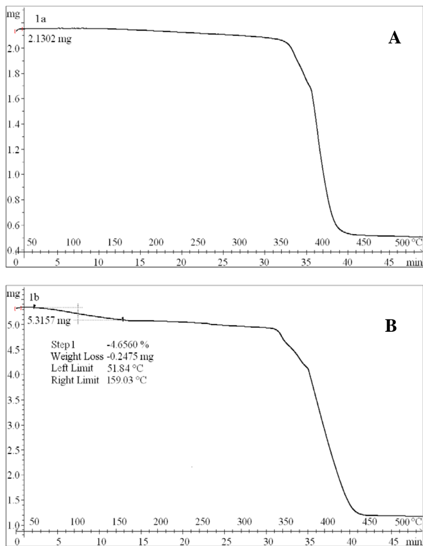
Figure S1 TGA curves of complexes 1a (S1A) and 1b (S1B).
