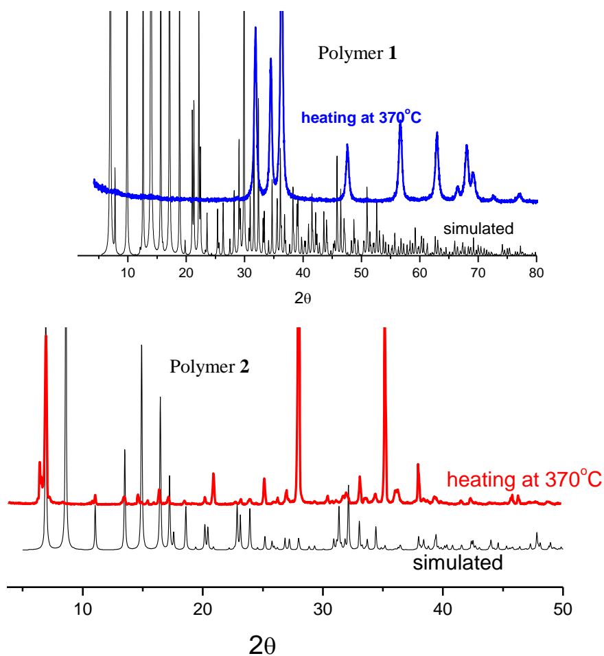
Figure S1. The XRD patterns after the samples heated at 370°C for one day and the XRD patterns simulated from the single crystal data.
