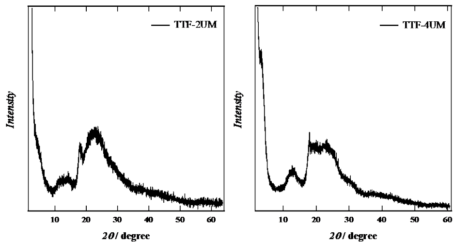
Fig. S1. XRD diffraction patterns of TTF-2UM and TTF-4UM.
