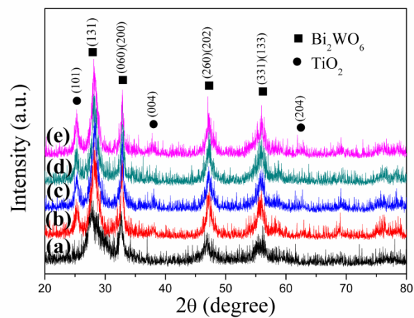
Figure S1. XRD patterns of \text{TiO}_2/\text{Bi}_2\text{WO}_6 heterostructure obtained for different reaction time: (a) 1h, (b) 7h, (c) 14h, (d) 21h, (e) 28h.
