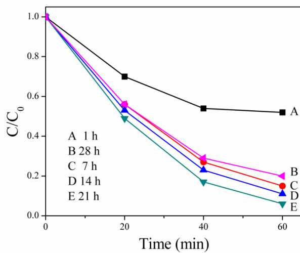
Figure S2. Degradation of RhB in presence of samples obtained for different reaction time: (A) 1h, (B) 28h, (C) 7h, (D) 14h, (E) 21h.
