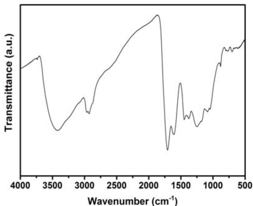
Figure S2. FTIR spectra of \text{SO}_3\text{H} -group functionalized carbon residual sample obtained by dissolving iron oxide in the \text{Fe}_3\text{O}_4@\text{C}-\text{SO}_3\text{H} sample.
