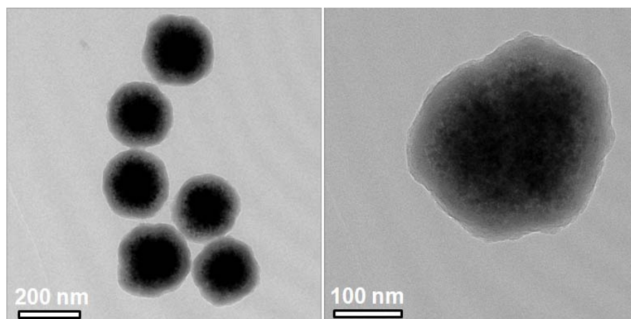
Figure S1. HRTEM images of \text{Fe}_3\text{O}_4@\text{C}-\text{SO}_3\text{H} MNPs.
