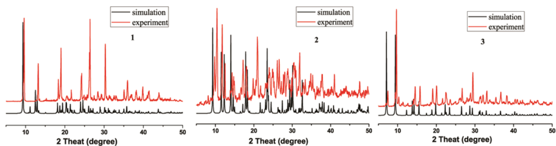
Figure S1. XRD patterns for compounds 1-3 .
