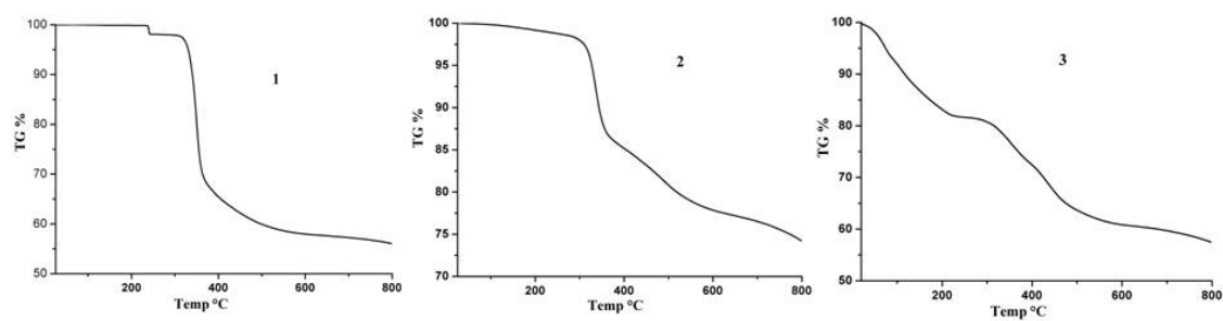
Figure S3. TG curves for compounds 1-3 .
