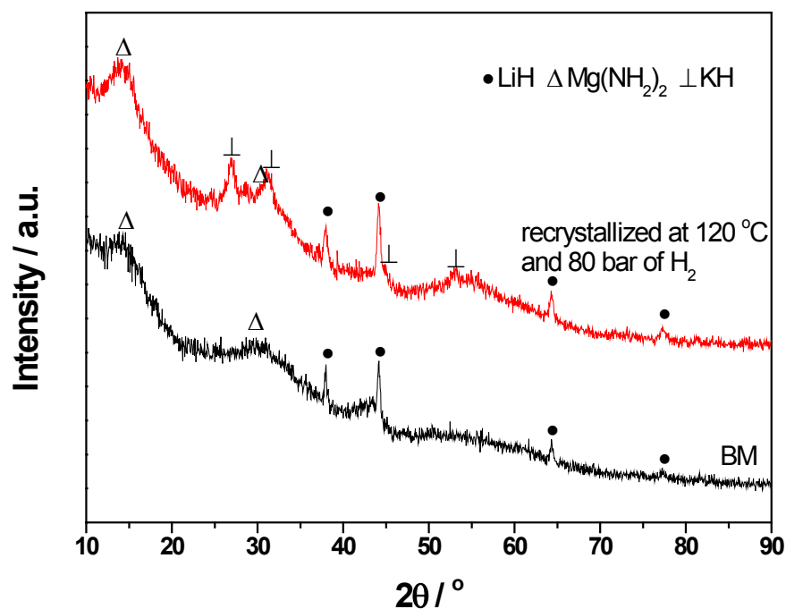
Fig. S1 XRD patterns of the Mg(NH 2 ) 2 -2LiH-0.08KH samples after milling and recrystallization.
