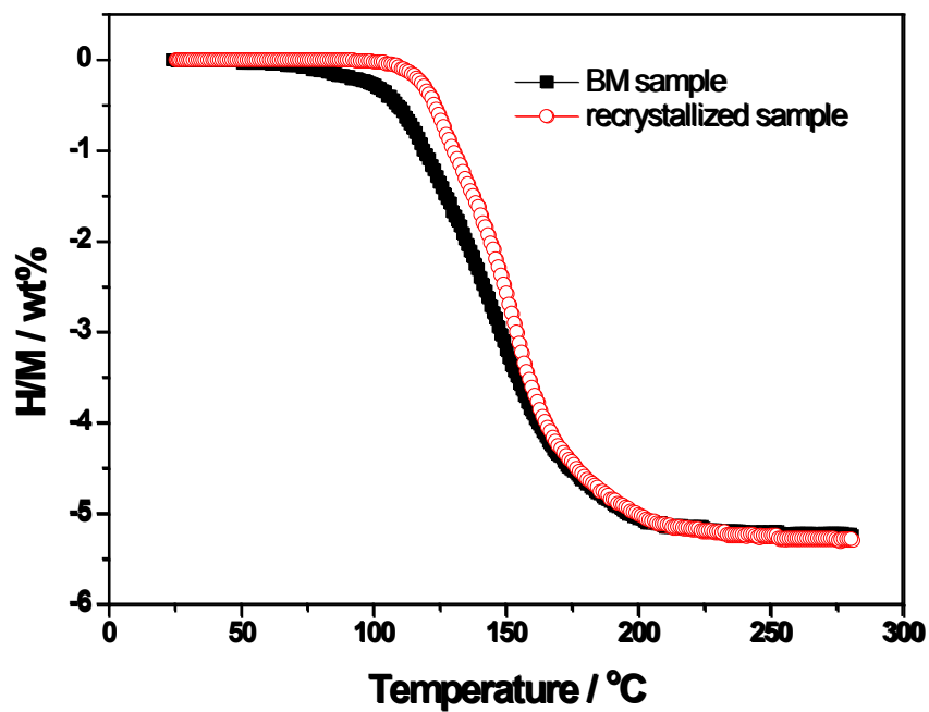
Fig. S2 Volumetric release curves of the Mg(NH 2 ) 2 -2LiH-0.08KH samples after milling and recrystallization.
