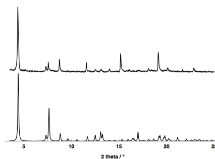
Figure S2: Comparison of the simulated from the single crystal data (bottom) and recorded (top) PXRD patterns for 1-AgSbF 6 .
