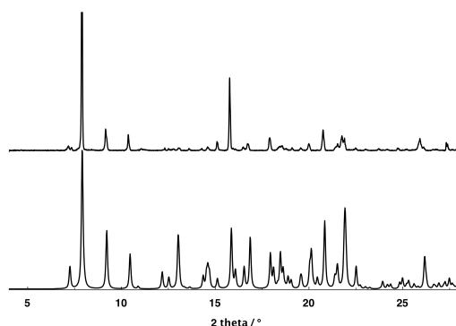
Figure S1: Comparison of the simulated from the single crystal data (bottom) and recorded (top) PXRD patterns for 1-AgBF 4 .
