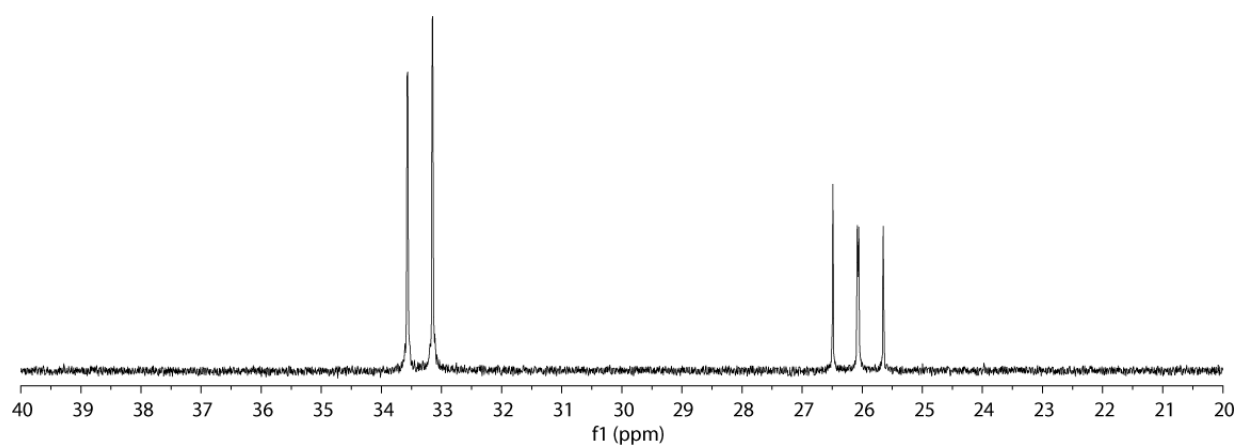
Figure S2. ^{31}\text{P}\{^1\text{H}\} NMR spectrum of 2 ( \text{CD}_2\text{Cl}_2 , 298 K).
