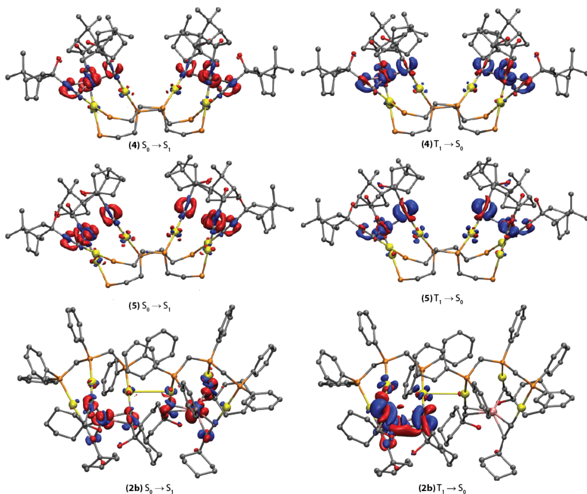
Figure S15. Electron density difference plots for the lowest energy singlet excitation ( S_0 \rightarrow S_1 ) and the lowest energy triplet emission ( T_1 \rightarrow S_0 ) of the Au^I-M^I complexes 4 and 5 , together with the dimeric structure 2b (isovalue 0.002 a.u.). During the electronic transition, the electron density increases in the blue areas and decreases in the red areas. Hydrogen atoms and phosphine-based Ph rings omitted for clarity.
