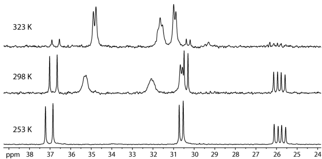
Figure S10. VT ^{31}\text{P} NMR spectra of 5 (acetone- d_6 ).
