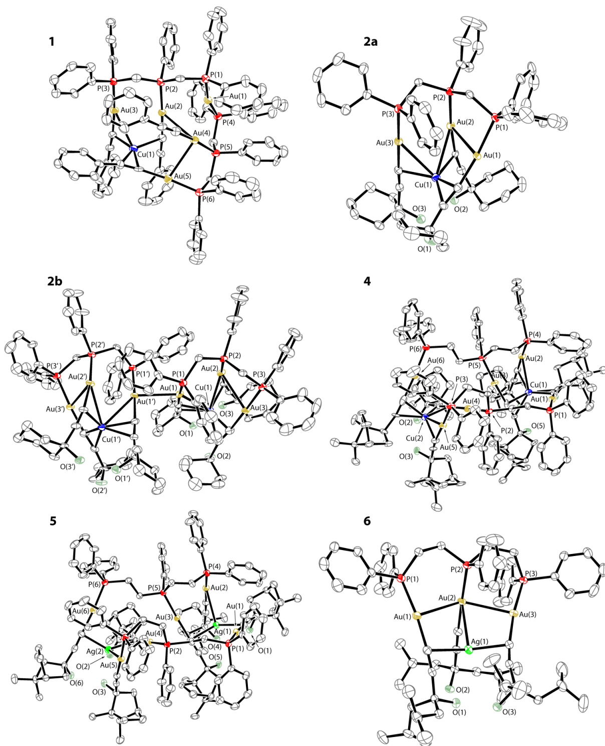
Figure S1. ORTEP views of the clusters 1, 2, 4–6.
