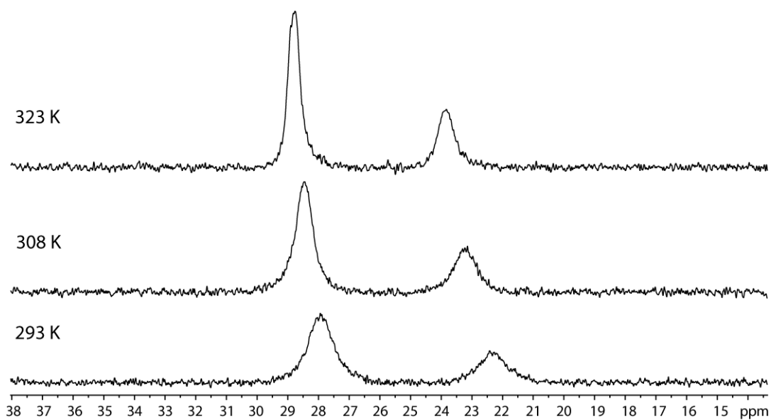
Figure S5. VT ^{31}\text{P} NMR spectra of 6 ( \text{acetone-}d_6 ).
