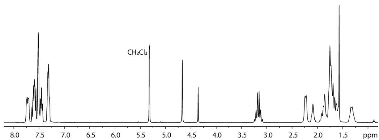
Figure S3. ^1\text{H} NMR spectrum of 2 ( \text{CD}_2\text{Cl}_2 , 298 K).
