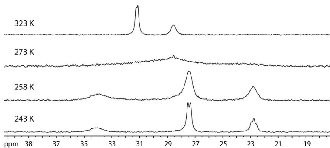
Figure S13. VT ^{31}\text{P}\{^1\text{H}\} NMR spectra of 3 (acetone- d_6 ).
