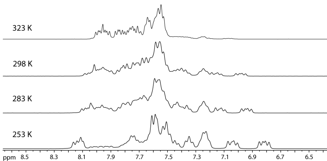
Figure S7. VT ^1\text{H} NMR spectra of 4 (acetone- d_6 ).
