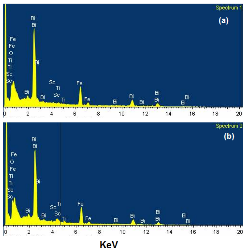
Figure S1: EDX spectra of (a) \text{BiFe}_{0.925}\text{Sc}_{0.05}\text{Ti}_{0.025}\text{O}_3 and (b) \text{BiFe}_{0.9}\text{Sc}_{0.05}\text{Ti}_{0.05}\text{O}_3 .
