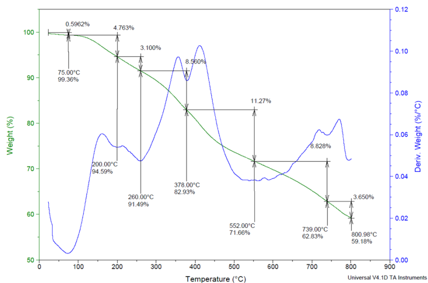
Figure S3. TGA of SWCNT-COOH 8.
