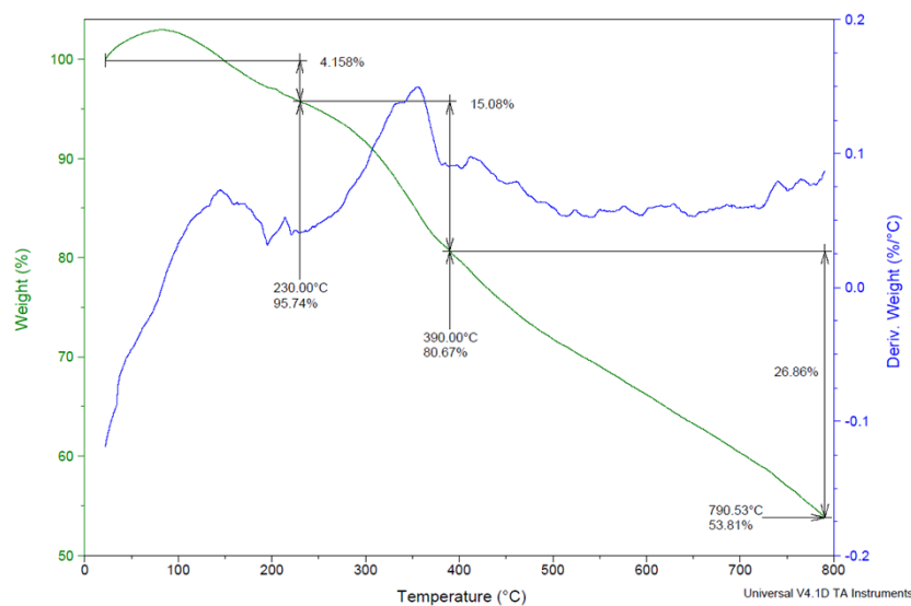
Figure S2. TGA of Pd(II)(bipyridyl)-SWCNT 7.
