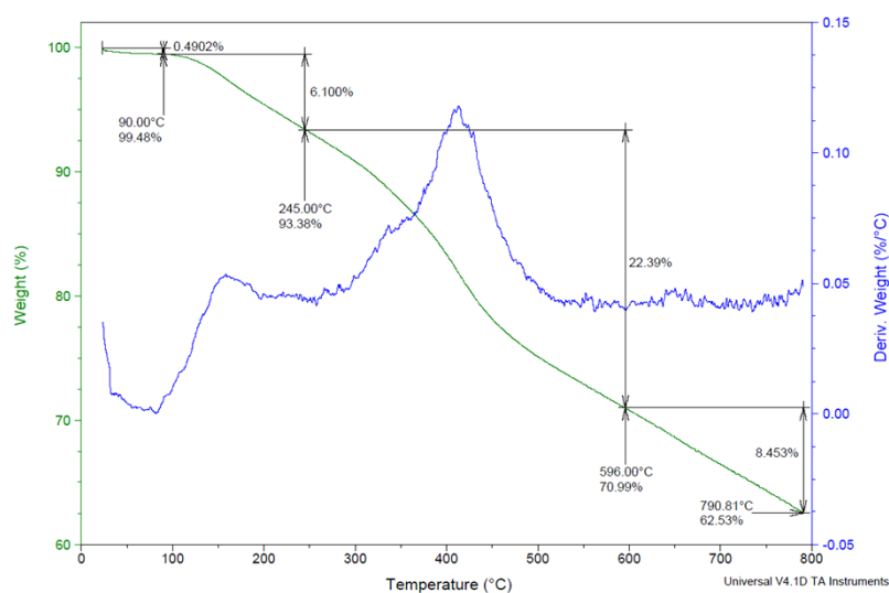
Figure S1. TGA of SWCNT-COOH 6.
