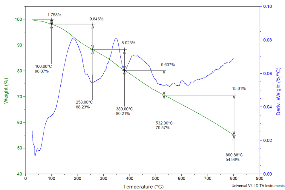
Figure S4. TGA of Ru(II)(bipyridyl)-SWCNT 9.
