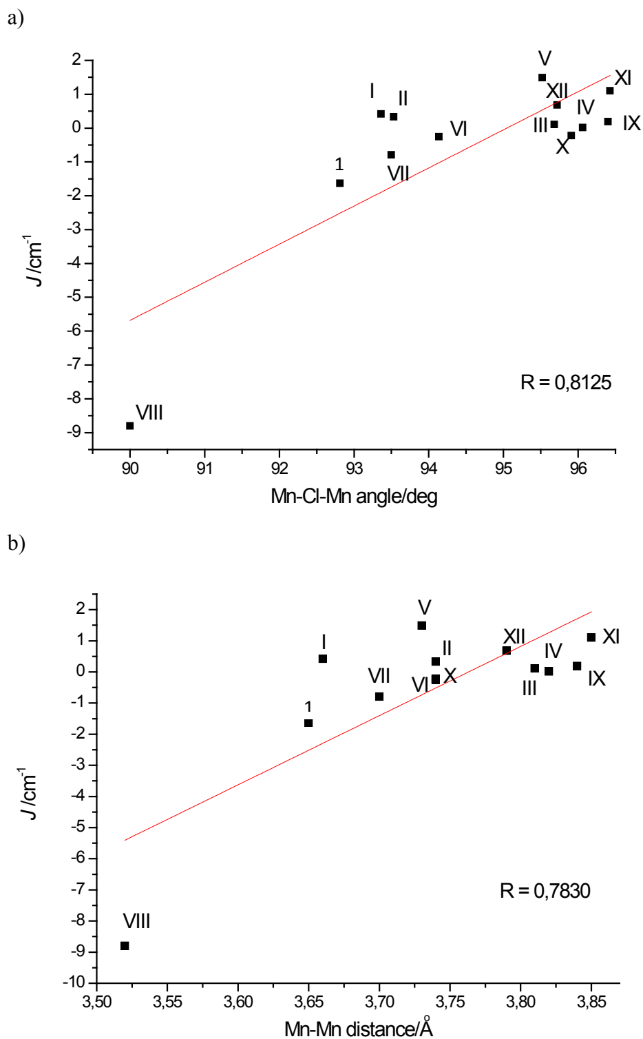
Fig. S1 Plots of J ( \text{cm}^{-1} ) versus various parameters 17 . (a) J ( \text{cm}^{-1} ) versus the Mn-Cl-Mn angle (deg). (b) J ( \text{cm}^{-1} ) versus the Mn···Mn distance (Å)
