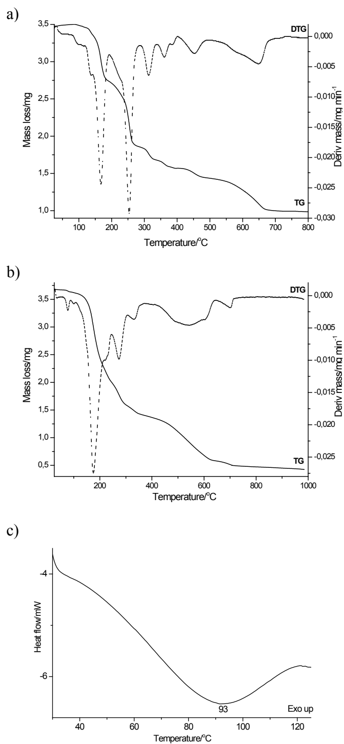
Fig. S2 TG/DTG of complex 1 (a), 2 (b), and DSC curves of complex 1 (c)
