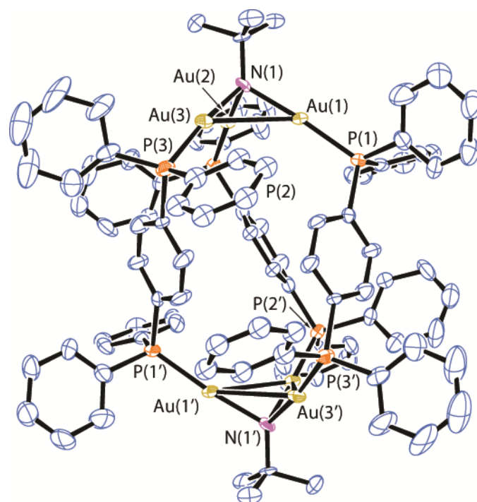
Figure S1. ORTEP view of the dication 1 (counterions and hydrogen atoms are omitted for clarity; ellipsoids are shown at 50% probability).
