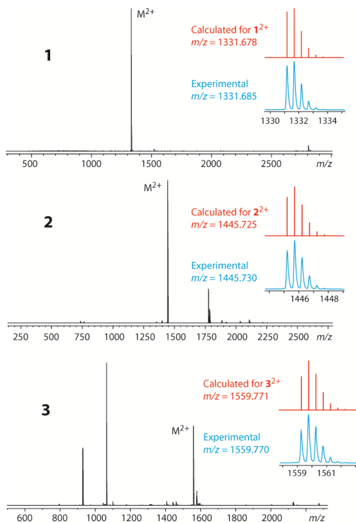
Figure S3. ESI-MS spectra of 1–3.
