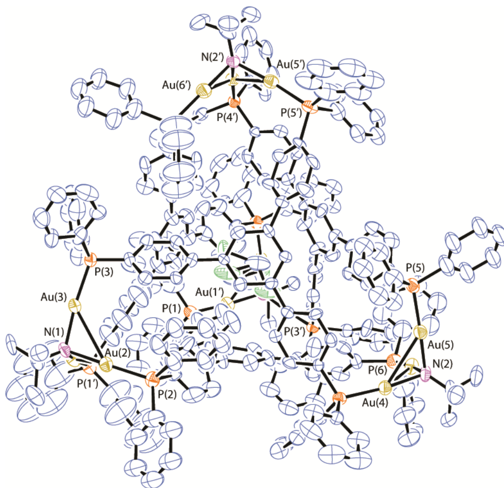
Figure S2. ORTEP view of the tetracation 4 (counterions and hydrogen atoms are omitted for clarity; ellipsoids are shown at 50% probability).
