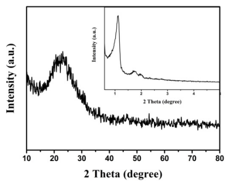
Figure 1. The XRD pattern of SBA-15 (Inset is the SAXRD pattern).
