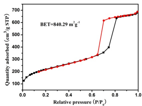
Figure 2. N 2 adsorption-desorption isotherms of SBA-15.
