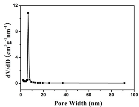
Figure 3. Pore size distribution of SBA-15.
