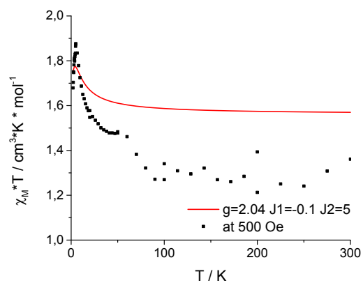
Figure 1: \chi T vs. T plot between 2 and 300 K for the tetranuclear Copper complex.
