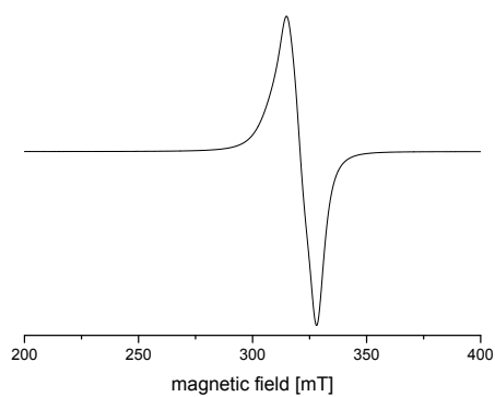
Figure 2: solid state EPR spectrum measured at 110 K.
