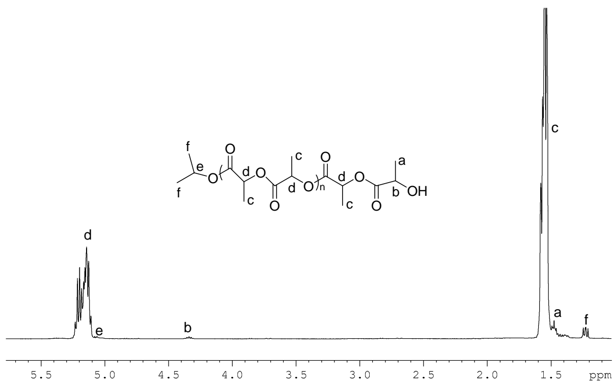
Figure S1. 1 H NMR spectrum (500 MHz, CDCl 3 ) of a polymer sample obtained from the 8 /isopropanol system with 8 /isopropanol/LA (mol/mol/mol) = 1/1/100 (Table 4, entry 3).
