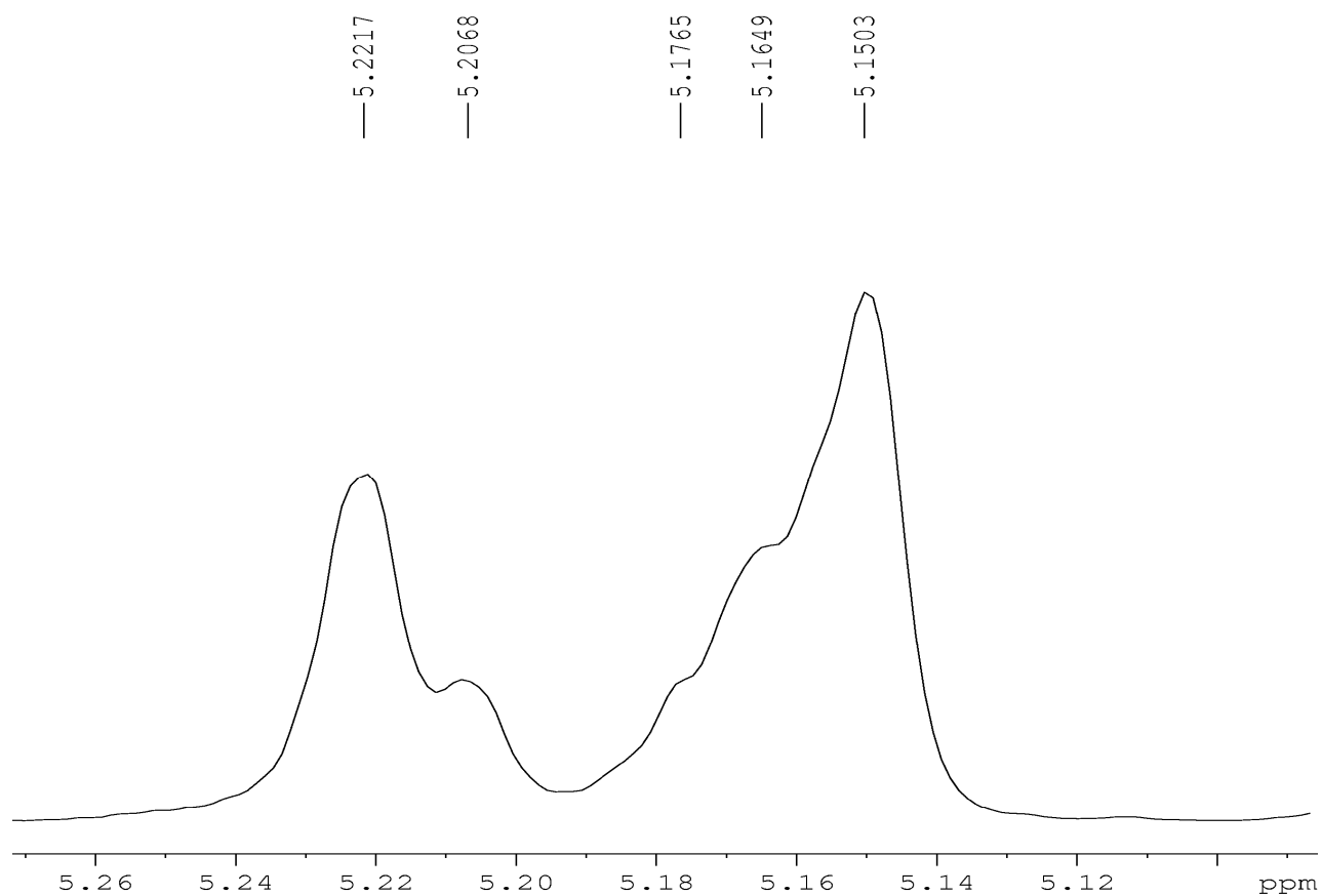
Figure S2. Decoupled ^1\text{H} NMR spectrum (500 MHz, \text{CDCl}_3 ) of a polymer sample obtained from the 8 /isopropanol system with 8 /isopropanol/LA (mol/mol/mol) = 1/1/100 (Table 4, entry 3).
