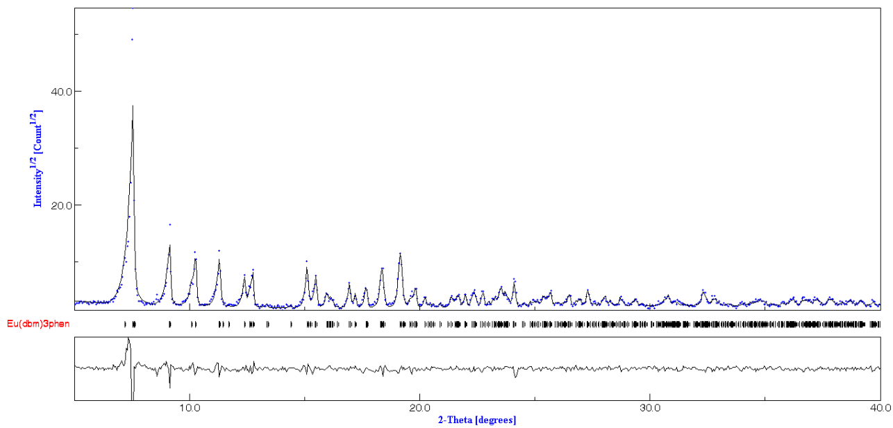
Figure S1: Rietveld refinement performed on the Eu(dbm)3phen diffractogram.
