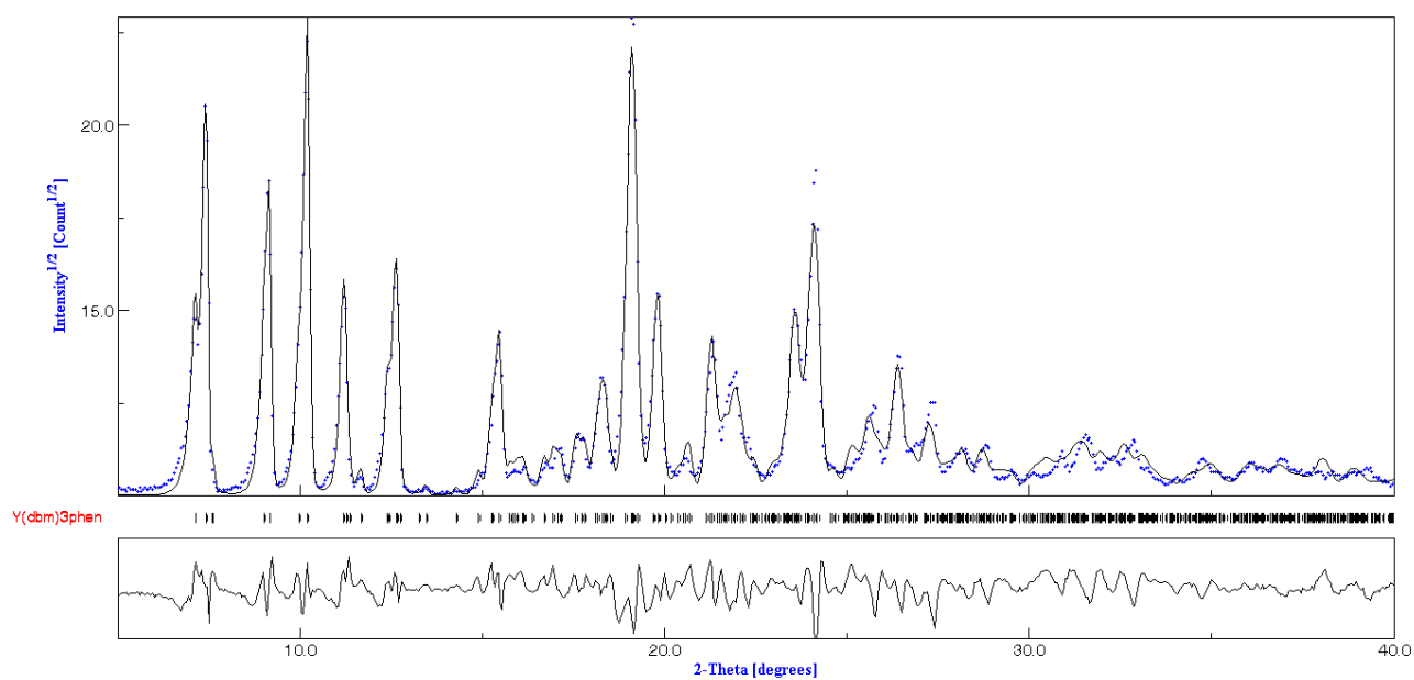
Figure S2: Rietveld refinement performed on the Y(dbm)3phen diffractogram.
