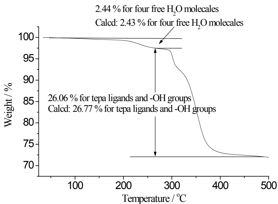
Fig. S1 Thermogravimetric analyses curve of 3 .
