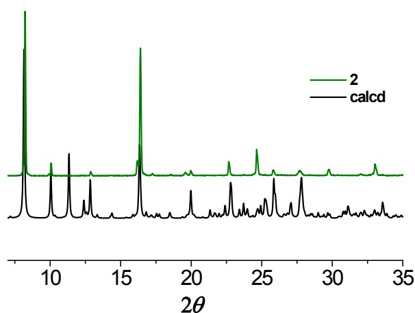
Fig. S2 The XRD patterns calculated from the single crystal data of 2 and observed for 2 .
