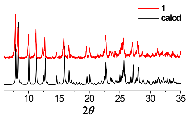
Fig. S1 The XRD patterns calculated from the single crystal data of 1 and observed for 1 .
