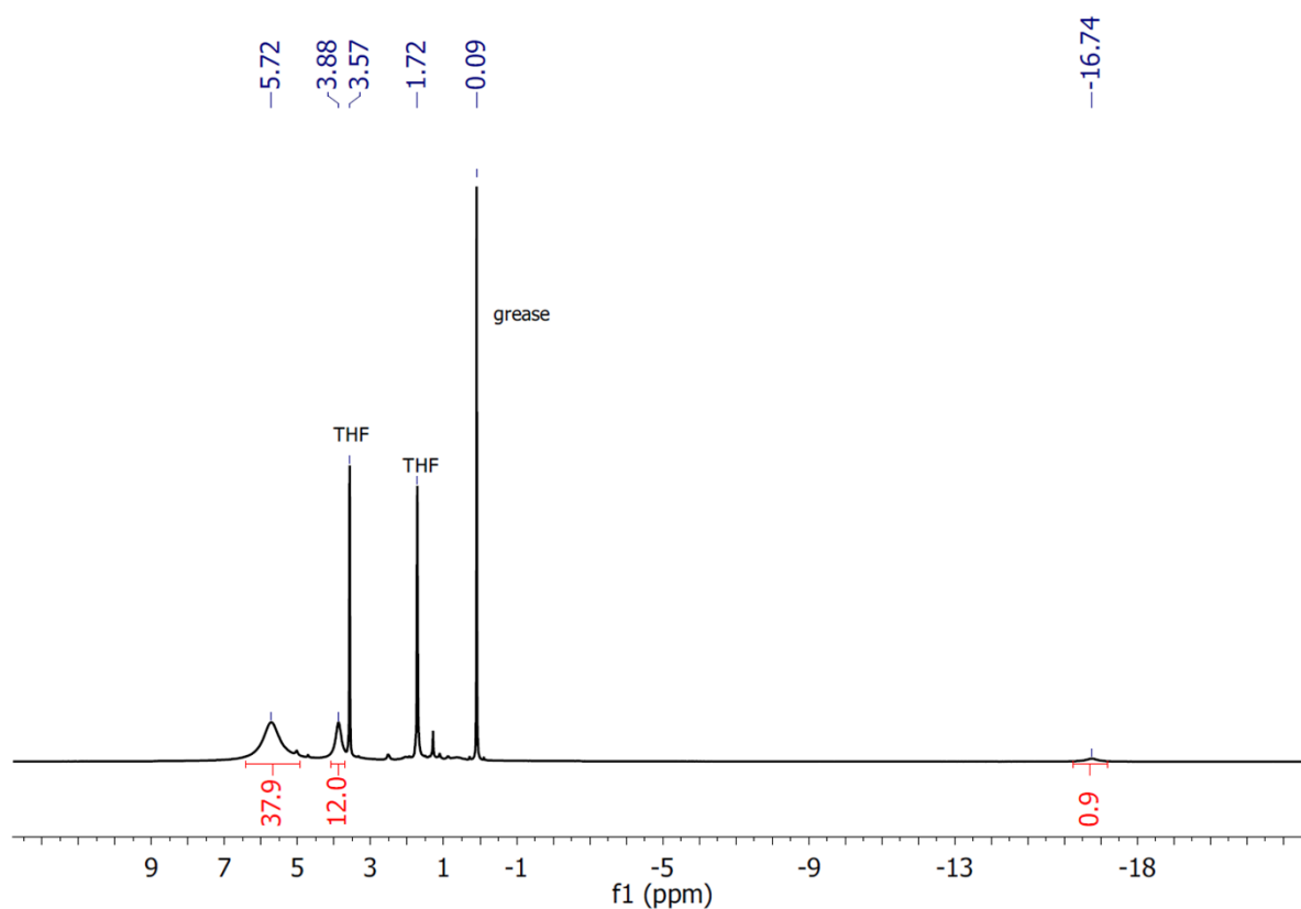
Figure S1. ^1\text{H-NMR} spectrum of the paramagnetic [(\text{acac})_2\text{Cu}_2(\text{NtBu})_4\text{S}] ( 3 ) depicting the presence of silicon joint grease.
