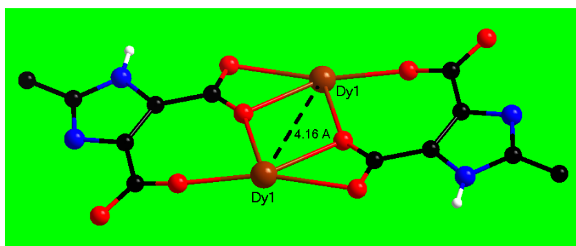
Fig. S5. Illustration of two adjacent Dy(III) ions doubly connected by 4-carboxylic group from Hmimda ligands viewed approximately down ac plane in 6 .
