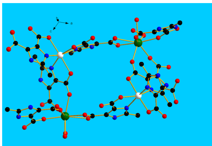
Fig. S4. Illustration of an individual \text{Ho}_2\text{Zn}_2 parallelogram fragment linked by Hmimda ligands viewed approximately down the bc plane in 2 . Color codes: Ho(III), green; Zn, white.
