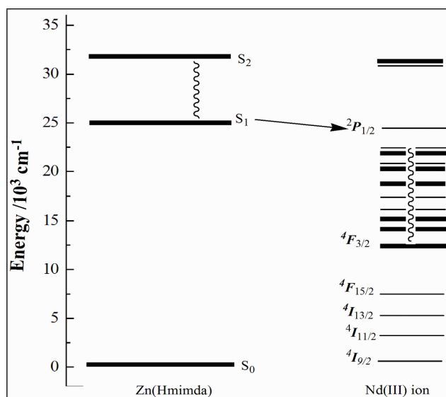
Fig. S12. Schematic representation of the energy flow paths during g sensitization of Nd(III) ion luminescence via the [Zn-Hmimda] unit.
