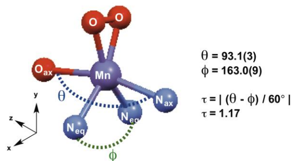
Figure S8. Calculation of \tau parameter for [Mn III (O 2 )(Tp Ph2 )]. For clarity, only the primary coordination sphere of Mn, N, and O is shown.
