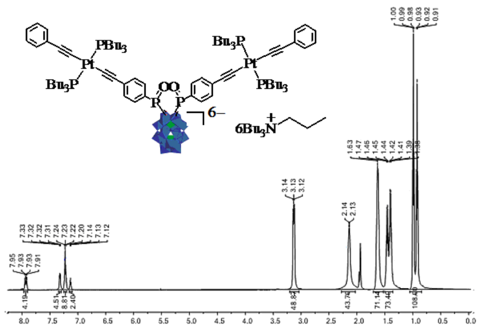
Fig. S1 ^1\text{H} NMR spectrum of 2PtOD in \text{CD}_3\text{CN} .
