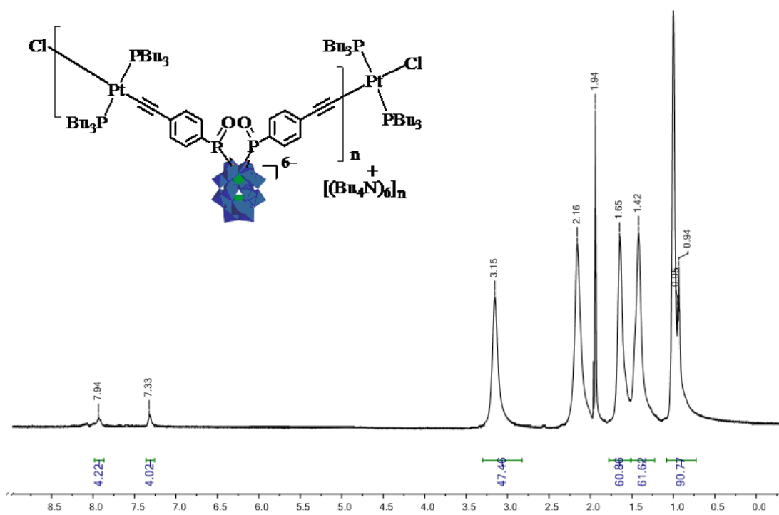
Fig. S2 ^1\text{H} NMR spectrum of PPtOD in \text{CD}_3\text{CN}
