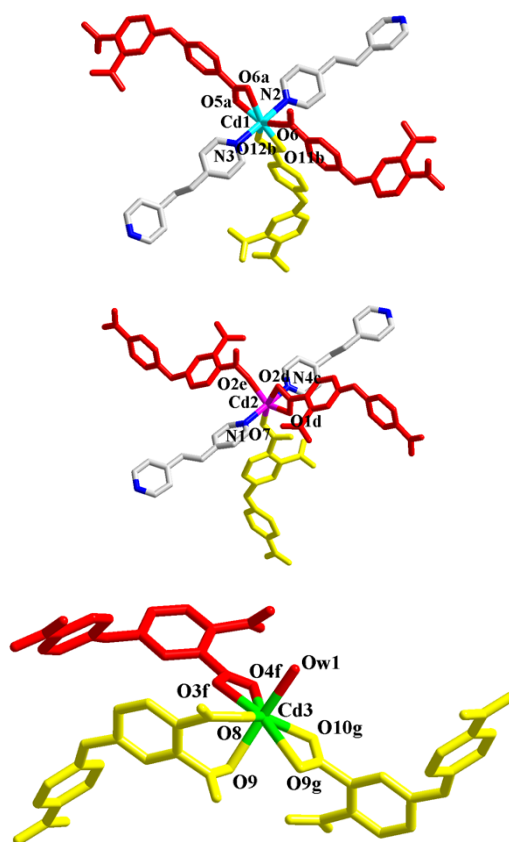
Fig. S1 Coordination environments around Cd1, Cd2 and Cd3 in 1 .
