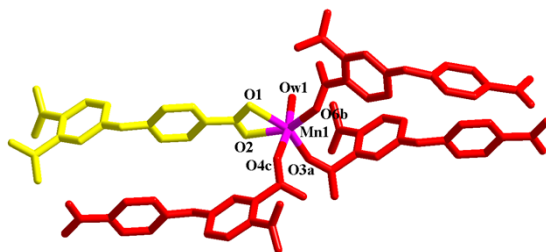
Fig. S3 Coordination environment around Mn1 in 2 .
