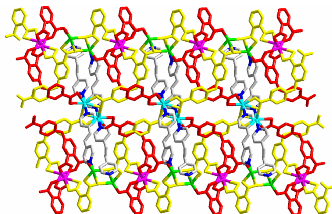
Fig. S2 3-D network of 1 .
