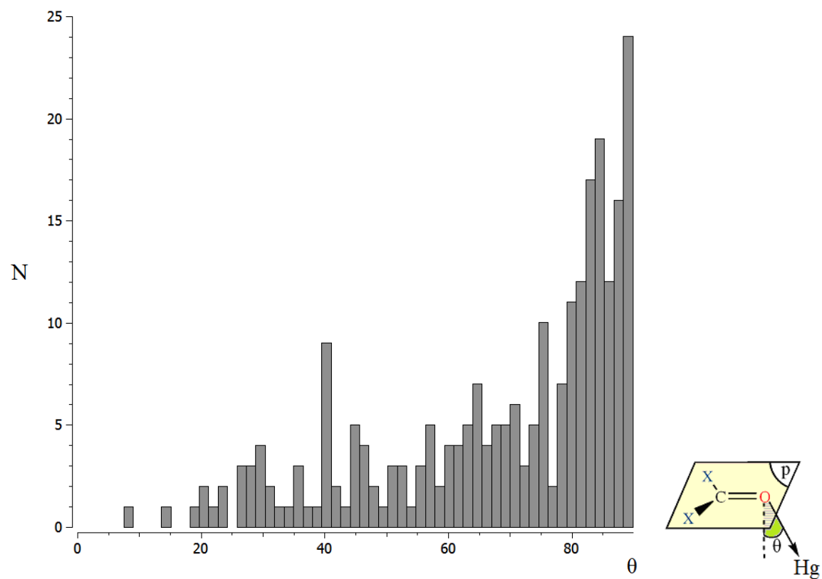
Figure S1. Histogram for the angle ( \theta , °) between the plane (containing (X)_2C=O moiety) normal and Hg-O vector from a CSD search without any filtrations. X stands for any atom.
