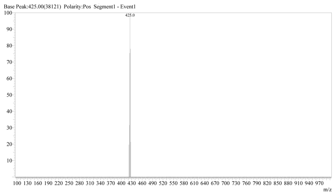
Fig. S1 ES-MS spectrum of complex 1
