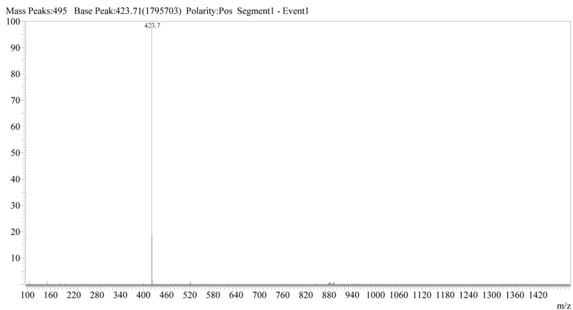
Fig. S10 ES-MS spectrum of complex 3 after co-incubated with glutathione under 37 °C for 1 h then R. T. for 24 h.
