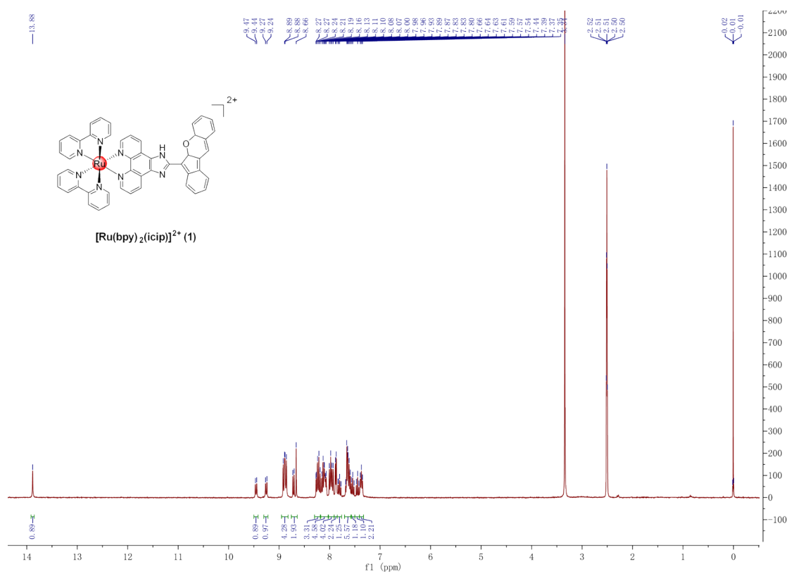
Fig. S2 ^1\text{H} NMR spectrum of complex 1
