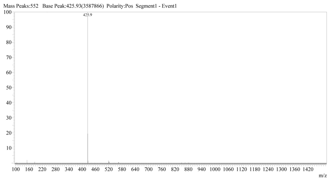
Fig. S4 ES-MS spectrum of complex 1 after co-incubated with glutathione under 37 °C for 1 h then R. T. for 24 h.
