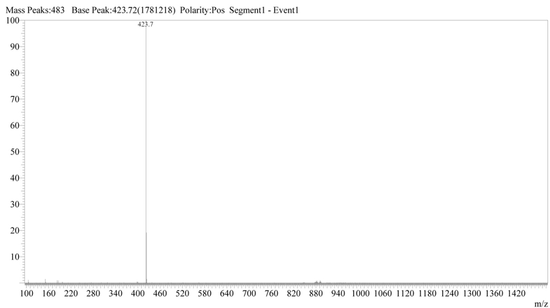
Fig. S9 ES-MS spectrum of complex 3 after co-incubated with L-cysteine under 37 °C for 1 h then R. T. for 24 h.
