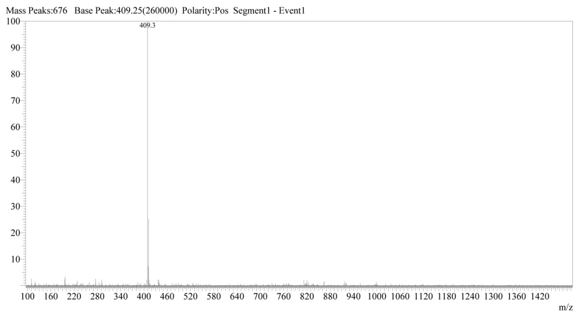
Fig. S7 ES-MS spectrum of complex 2 after co-incubated with glutathione under 37 °C for 1 h then R. T. for 24 h.
