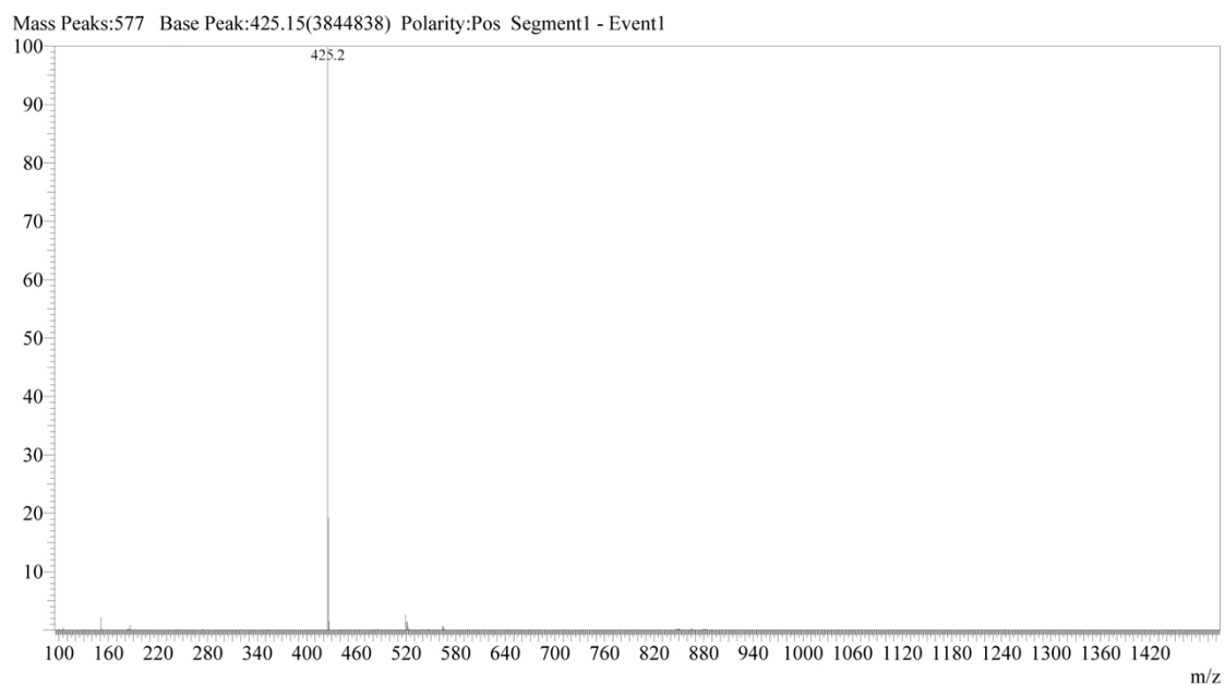
Fig. S3 ES-MS spectrum of complex 1 after co-incubated with L-cysteine under 37 °C for 1 h then R. T. for 24 h.
