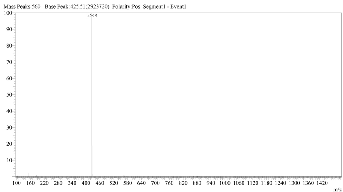
Fig. S5 ES-MS spectrum of complex 1 after co-incubated with dithiothreitol under 37 °C for 1 h then R. T. for 24 h.
