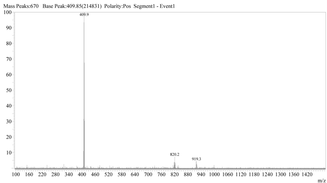
Fig. S6 ES-MS spectrum of complex 2 after co-incubated with L-cysteine under 37 °C for 1 h then R. T. for 24 h.
