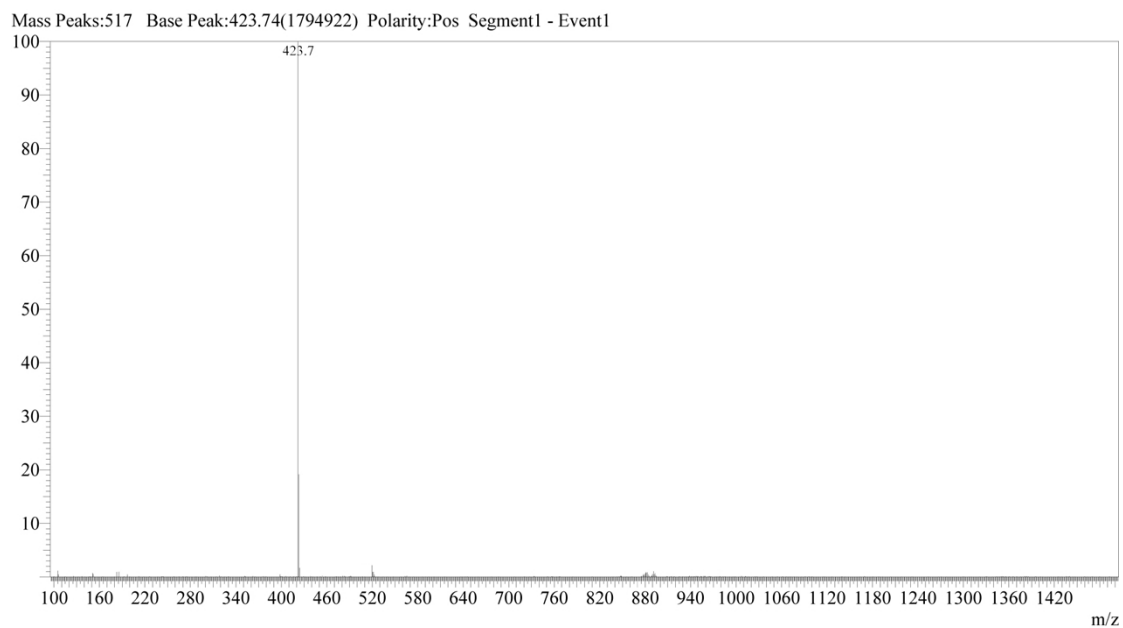
Fig. S1 ES-MS spectrum of complex 3 after co-incubated with dithiothreitol under 37 °C for 1 h then R. T. for 24 h.
