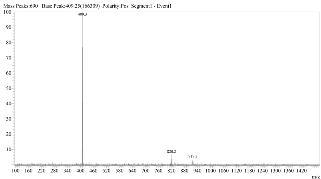
Fig. S8 ES-MS spectrum of complex 2 after co-incubated with dithiothreitol under 37 °C for 1 h then R. T. for 24 h.
