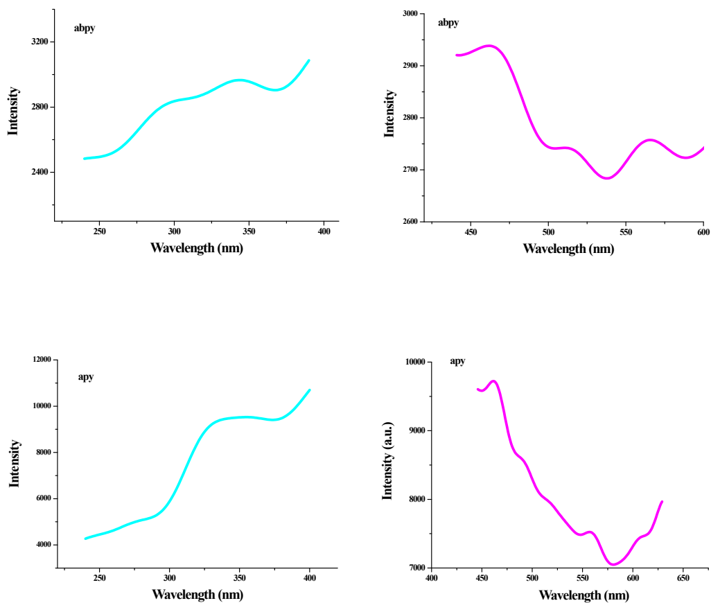
Fig. S4 Excitation (blue) and emission (pink) spectra of abpy and apy.
