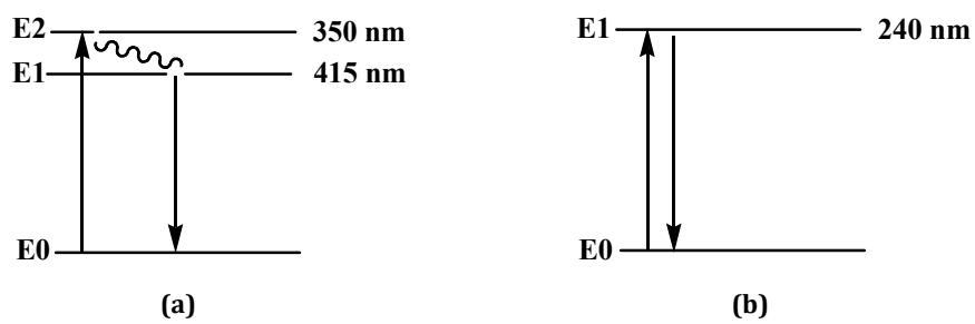
Fig. S6 Diagrams of energy levels for 1 (a) and 3 (b).
