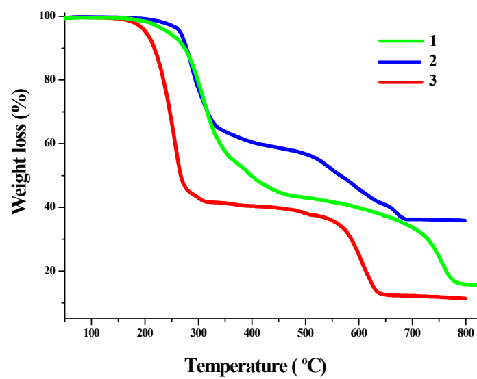
Fig. S2 TG curves of 1-3.
