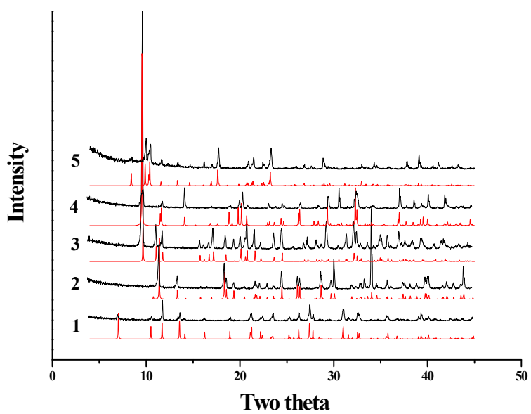
Fig. S3 Simulated (red) and experimental (black) powder XRD patterns of 1-5.
