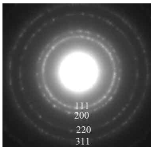
Fig S3 Selected-area electron diffractionhaves of Pt NFs
