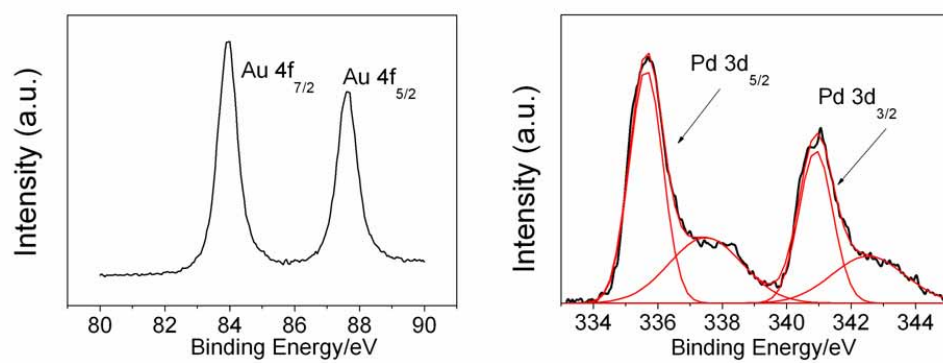
Figure S5: XPS data of Au 4f (A), and Pd 3d (B)
