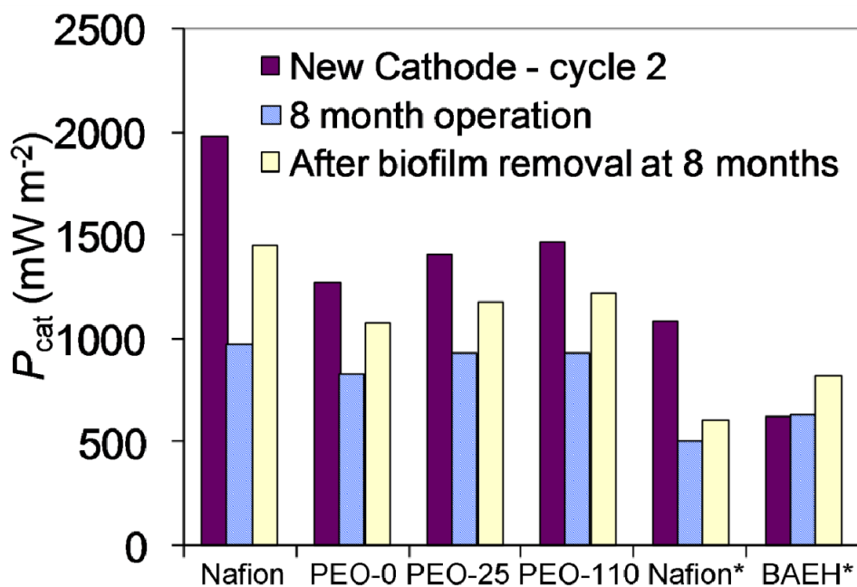
Fig. S2 MFC maximum power densities with new cathodes, cathodes containing biofilm, and cathodes where the biofilm had been removed. Nafion* and BAEH* contained 0.05 \text{ mg cm}^{-2} Pt whereas other cathodes contained 0.5 \text{ mg cm}^{-2} Pt. A MFC reactor with 0.5 \text{ mg cm}^{-2} Pt BAEH did not show stable results at 8 months.
