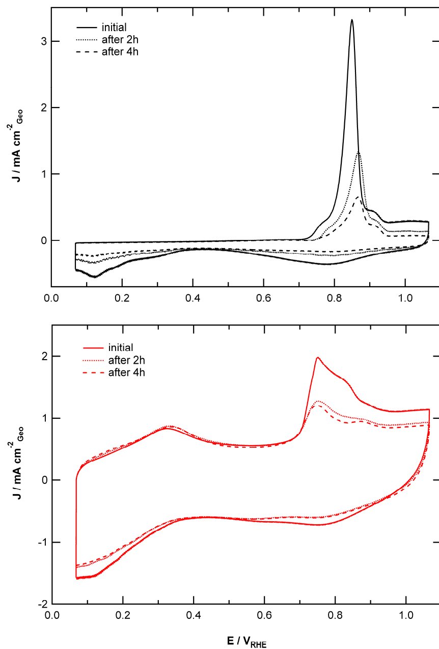
Figure S1. CO stripping curves of catalyst I (upper part) and catalyst II (lower part) in their initial state as well as after 2h and 4h accelerated degradation treatment. The treatment
