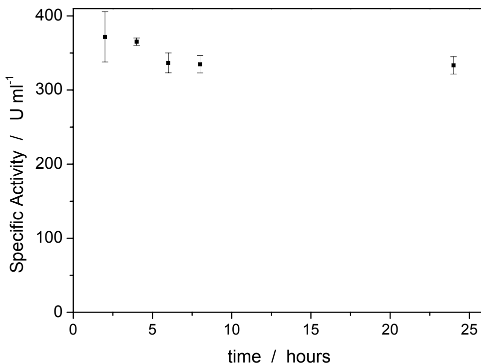
Figure S-1: Enzyme activity measured by UV-Vis spectroscopy for an enzyme sample kept constantly at 25°C at pH = 7.2. Details of enzymatic assay can be found in the experimental section of the main text.
